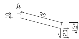
11-12. Underbleck 90
