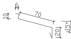
9-10. Underbleck 70
