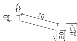
9-10. Underbleck 70
