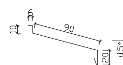
11-12. Underbleck 90
