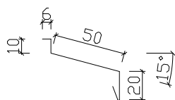
7-8. Underbleck 50
